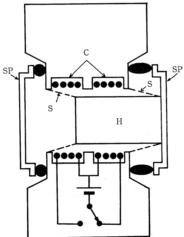
Fig. 4 Schematic diagram of P-S source. H: hammer, SP: vibration plate made by steel, C: solenoid coil, S: spring.
