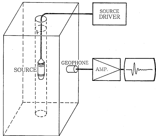
Fig.10 Comparative experiment in the test hole.
