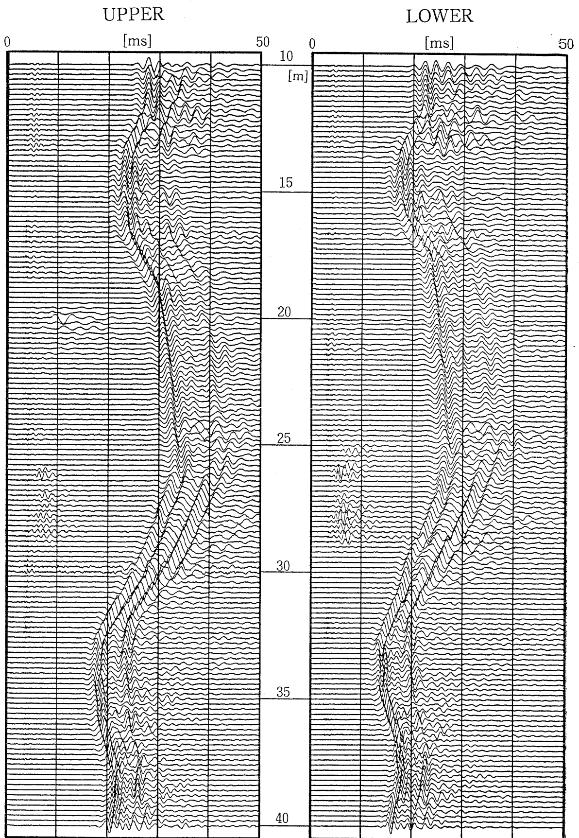
Fig.5 Record examples using P-S source.
