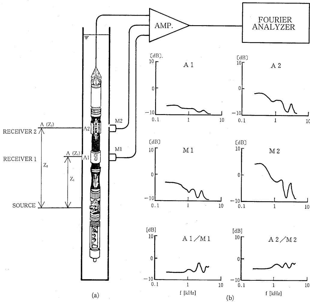
Fig. 14 (a) Schematic diagram of Suspension P-S Logging System. (b) Correction of system response
