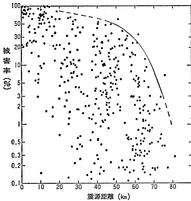
図-4-1 震源距離と被害率の関係：沖積低地 Fig. 4-1 Relationship between hypocentral distance and damage ratio: alluvial lowland.
