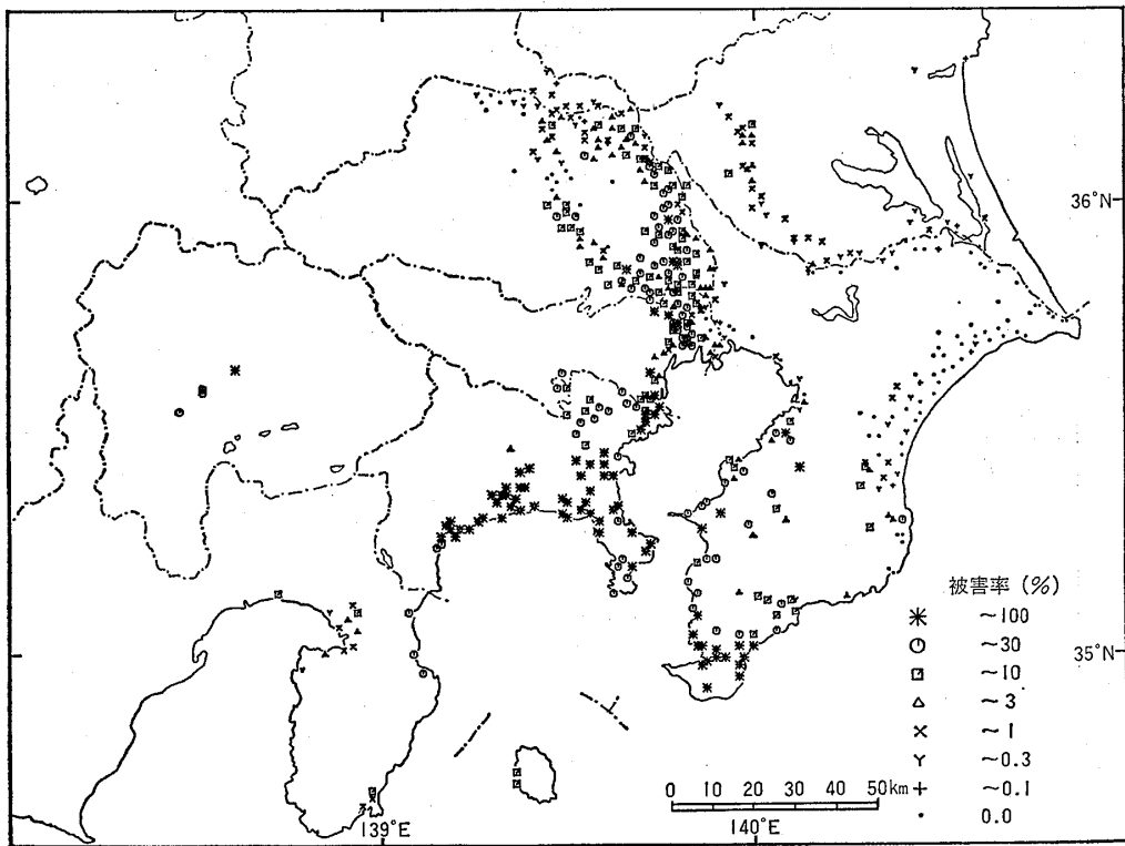
図一3-1 木造家屋被害率分布：沖積低地 Fig. 3-1 Distribution of ratio of damaged wooden houses: alluvial lowland.
