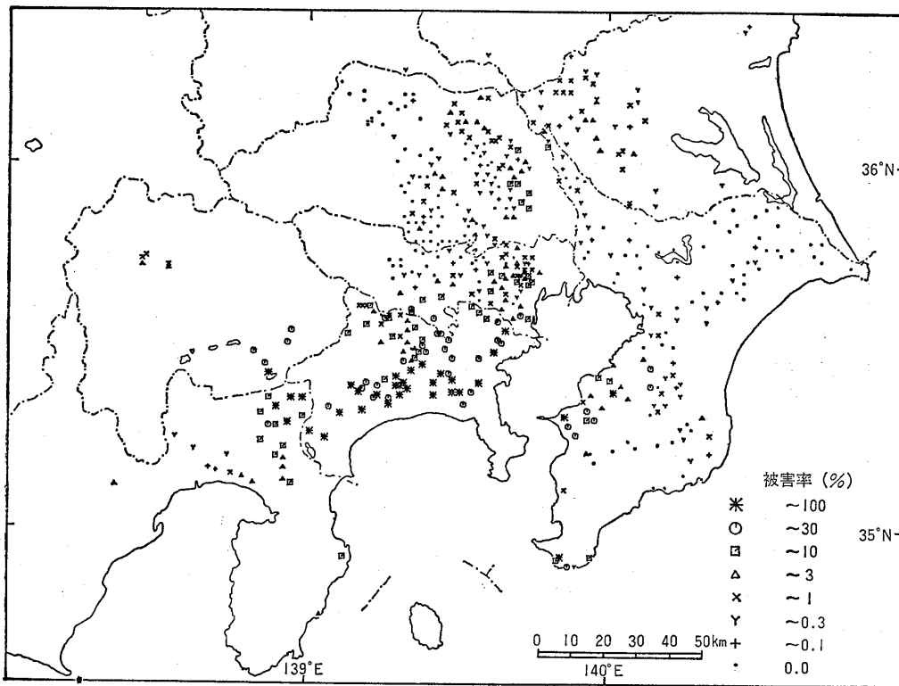
図-3-3 木造家屋被害率分布：台地 Fig. 3-3 Distribution of ratio of damaged wooden houses: terrace region.
