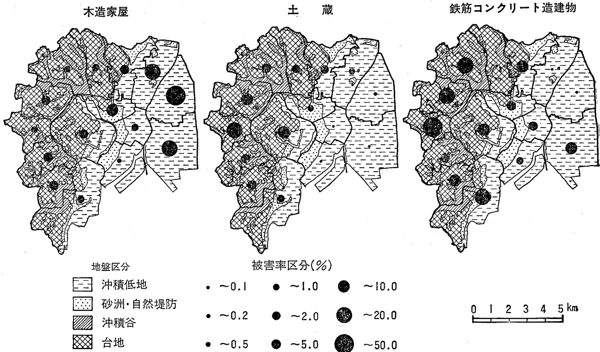
図一9 地盤と各種建物の被害率 Fig. 9 Ground type distribution and damage ratio of some kinds of structures.
