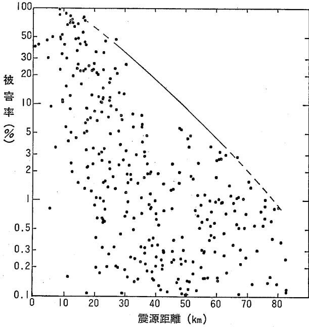
図-4-3 震源距離と被害率の関係：台地 Fig. 4-3 Relationship between hypocentral distance and damage ratio: terrace region.
