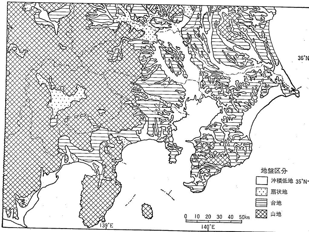
図-2 地盤区分図 Fig. 2 Distribution of ground type.
