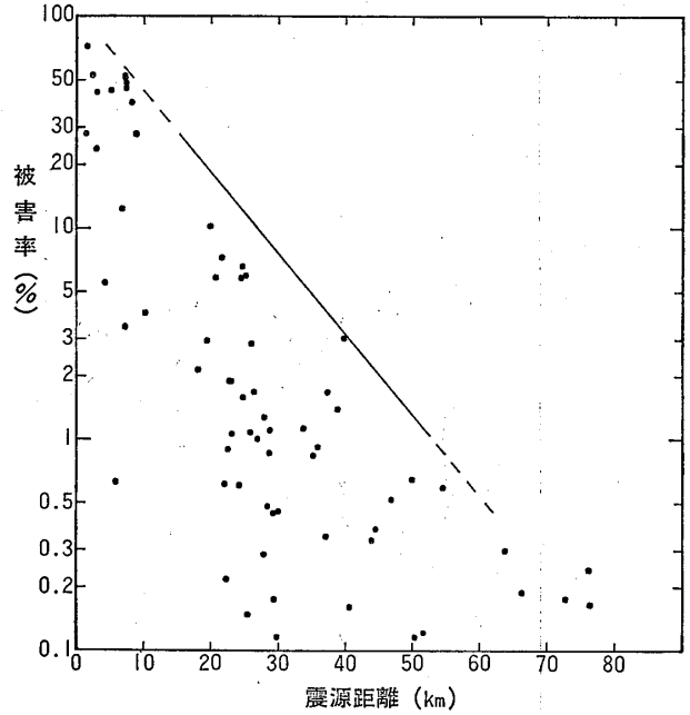
図-4-4 震源距離と被害率の関係：山地 Fig. 4-4 Relationship between hypocentral distance and damage ratio: mountainous region.
