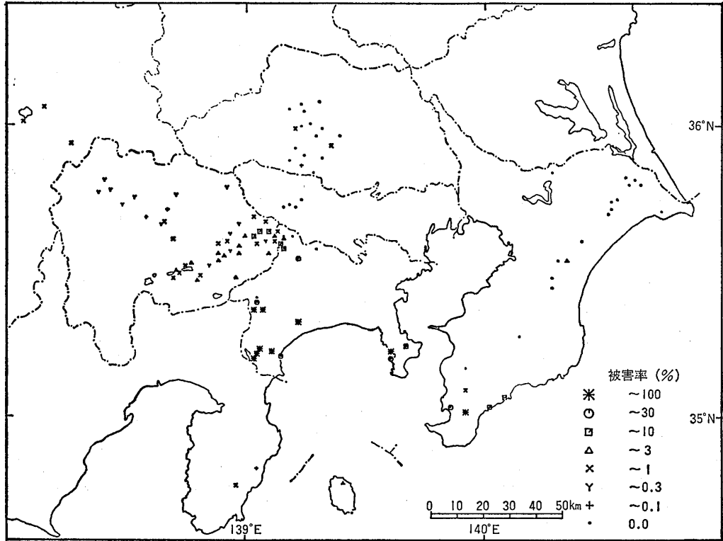
図-3-4 木造家屋被害率分布：山地 Fig. 3-4 Distribution of ratio of damaged wooden houses: mountaneous region.
