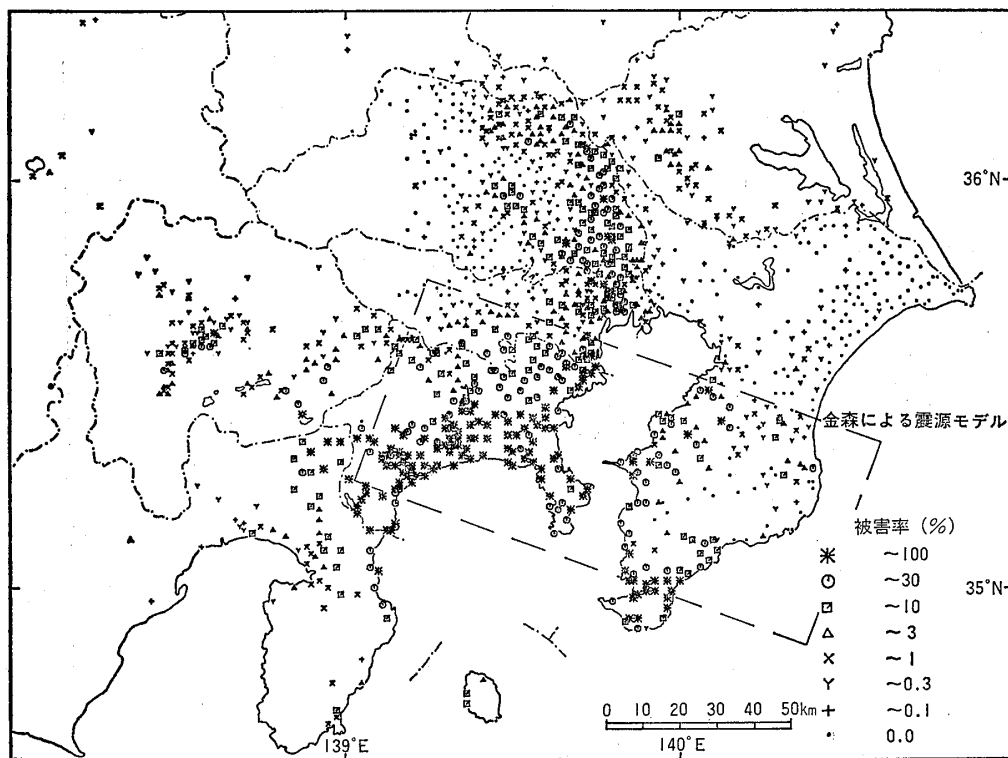
図一 1923年関東大地震による木造家屋被害率分布 Fig. 1 Distribution of ratio of damaged wooden houses due to 1923 Kanto Earthquake.
