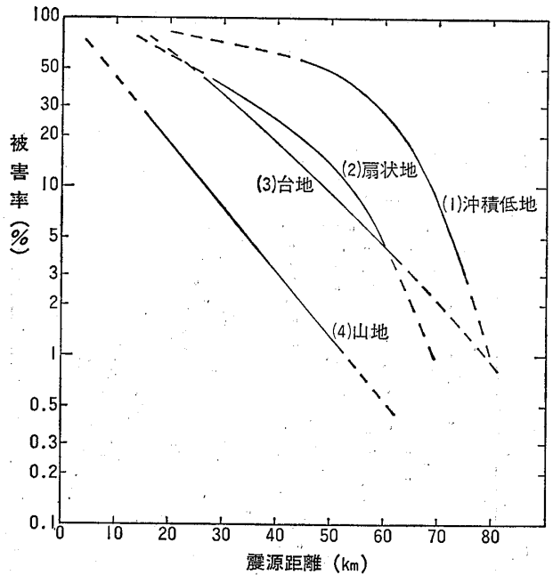
図-5 地盤区分による震源距離と被害率の関係 Fig. 5 Relationship between hypocentral distance and damage ratio due to ground type.
