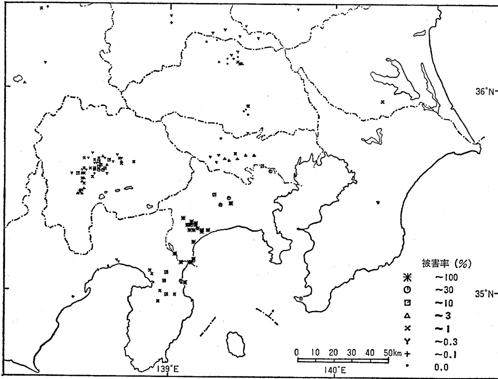
図-3-2 木造家屋被害率分布：扇状地 Fig. 3-2 Distribution of ratio of damaged wooden houses: fan region.
