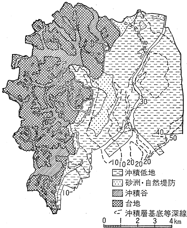
図一8 東京市域の地盤区分図 Fig. 8 Ground type distribution of Tokyo City.
