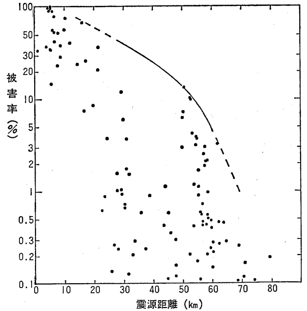
図-4-2 震源距離と被害率の関係：扇状地 Fig. 4-2 Relationship between hypocentral distance and damage ratio: fan region.
